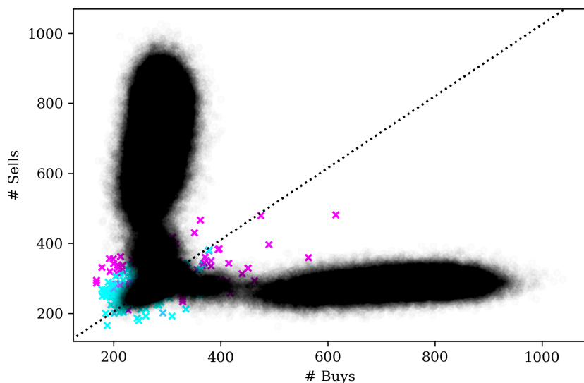
(c) XOM 1993
