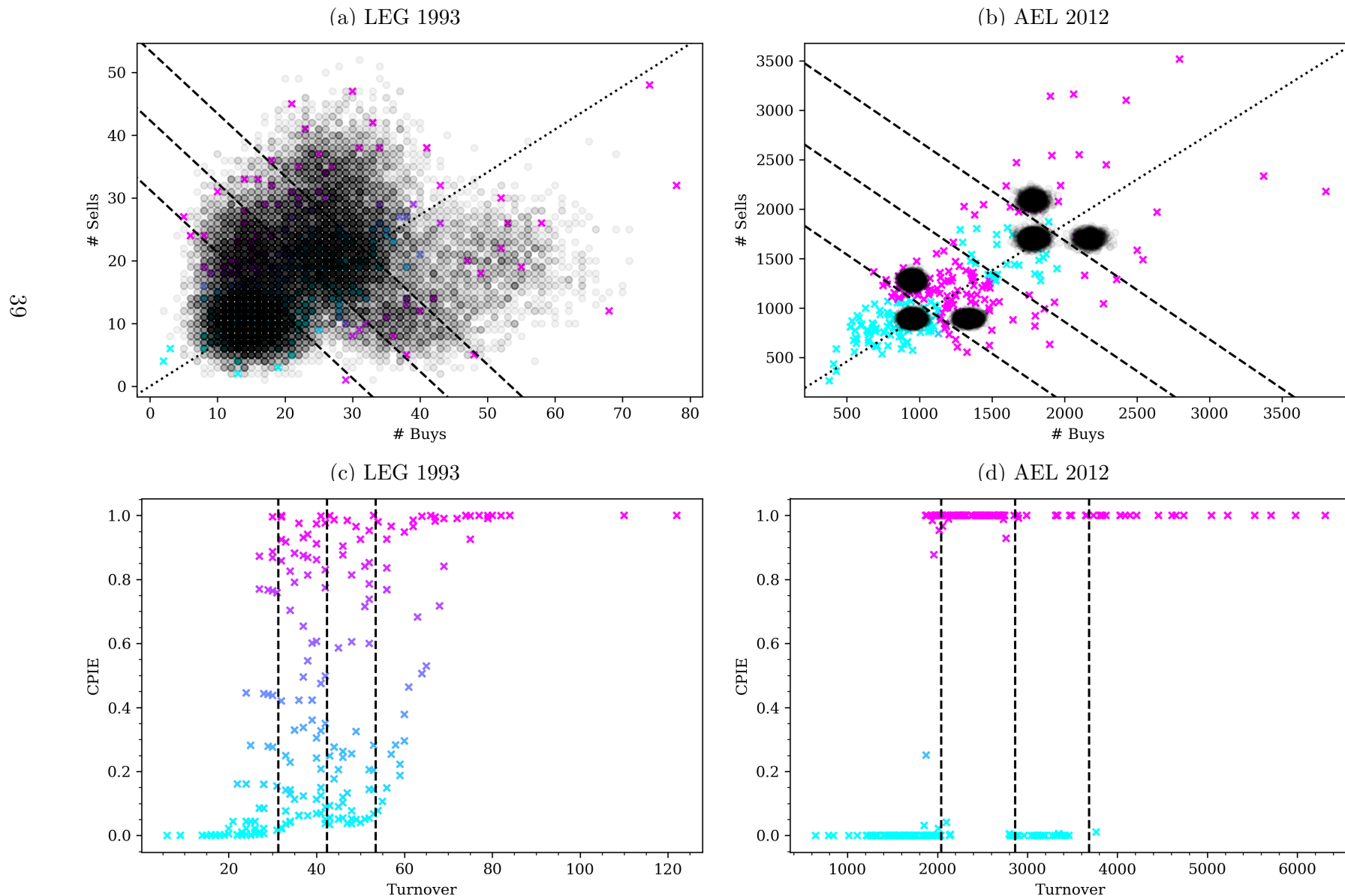
Figure A3: APIN Model Examples – 5% R^2 . This figure compares real and simulated data for Leggett & Platt Inc. (LEG) in 1993 and American Equity Life Investments (AEL) in 2012 from the APIN model. These stocks represent the 5% level of R^2 's in the cross-section, from a regression of CPIE_{APIN} on CPIE_{Mech,APIN} . In Panels A and B, the real data are marked as +. The real data are shaded according to the CPIE_{APIN} , with darker markers (+ magenta) representing high and lighter markers (+ cyan) low CPIE 's. High (low) probability states in the simulated data appear as a dark (light) “cloud” of points. Panels C and D plot the CPIE 's for the real data as a function of turnover along with a dashed line indicating the mean turnover.
