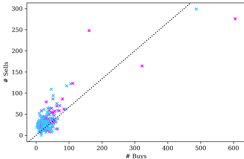
(c) USR 1993
