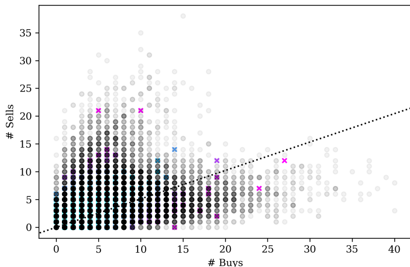
(c) LM 1993
