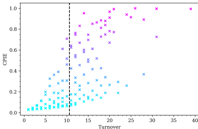
(c) LM 1993
